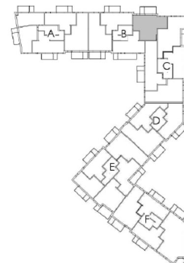
Plan 2-7
